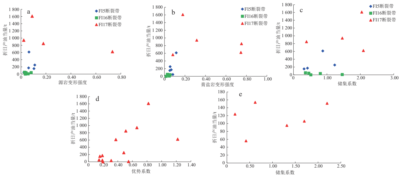
图 13 富满地区走滑断裂带运聚成藏要素对油气富集程度的影响 Fig. 13 Influence of factors controlling hydrocarbon migration and accumulation on hydrocarbon enrichment in strike-slip fault zones in the Fuman area a. 烃源岩层变形强度与折日产油气当量关系; b. 膏盐岩层变形强度与折日产油气当量关系; c. 储集系数与折日产油气当量关系; d. 垂向充注型油气藏优势系数与折日油气产量关系; e. 侧向运移调整主导型油气藏储集系数与折日产油当量关系
